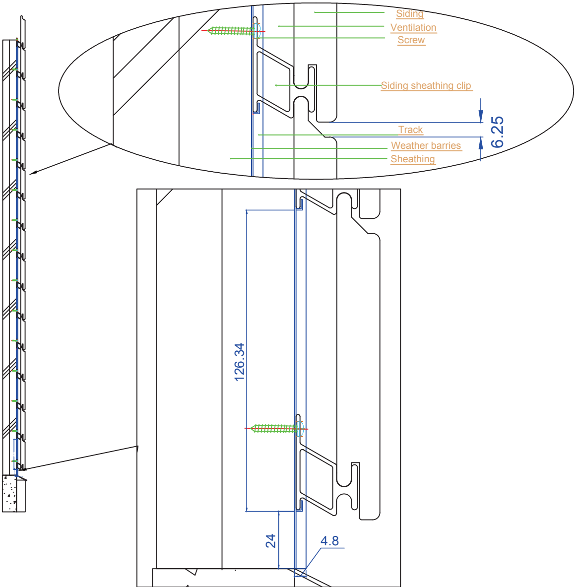
Installation Sheathing With Track
