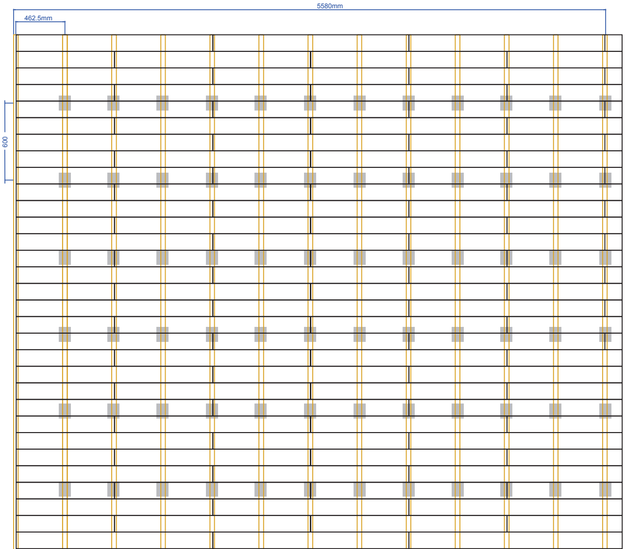
Staggered 462.5mm Center to Center
